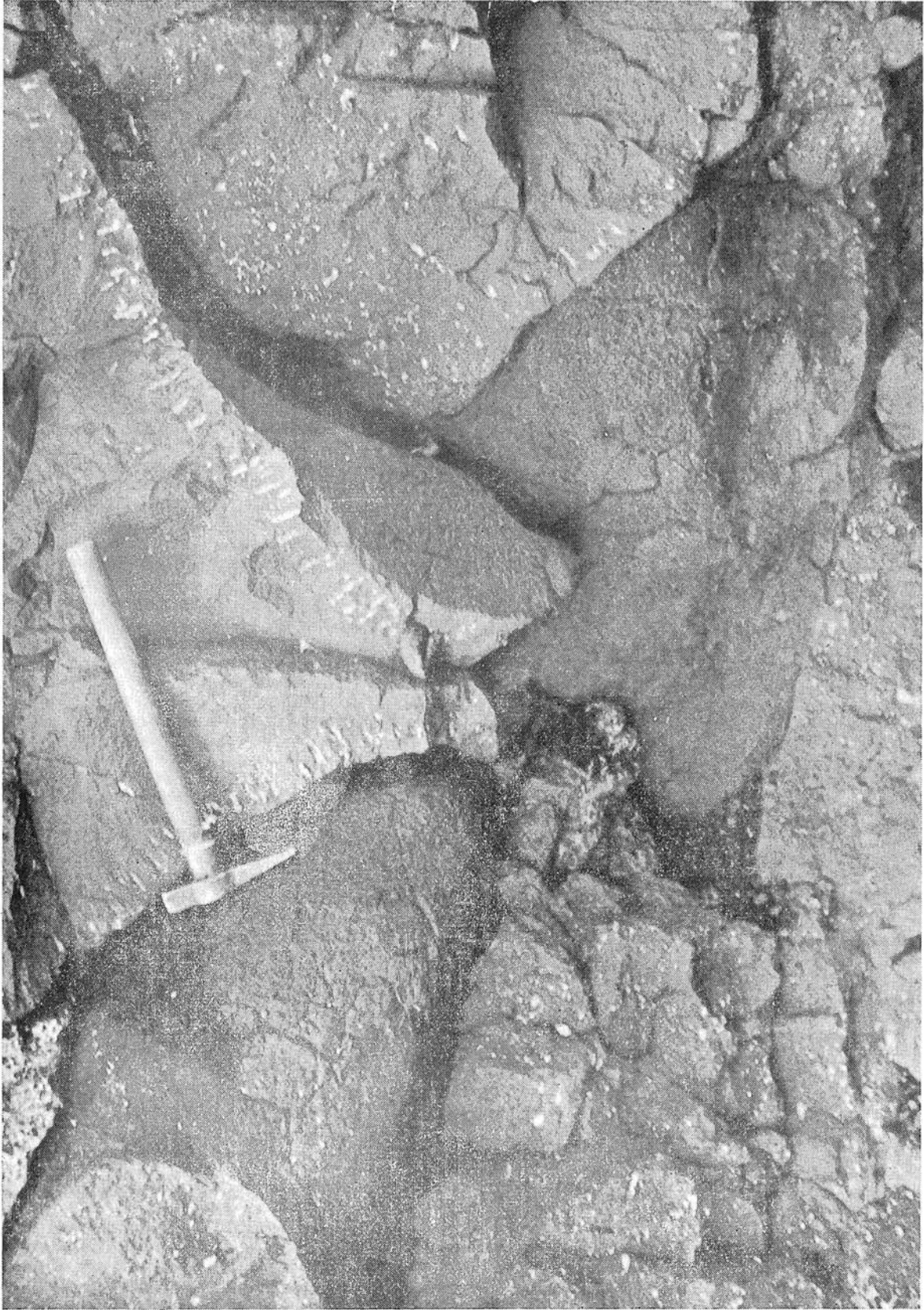
Levha V. Pilov Lavlar, Ulukışla. Plate V. Pillow Lavas, Ulukışla.
